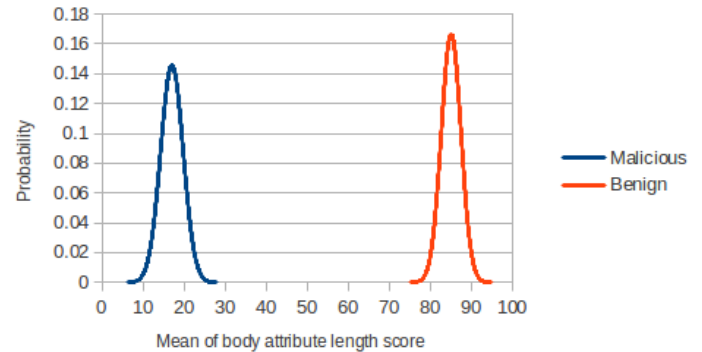
Figure 3: Normal distribution of the body_attrib_length feature
